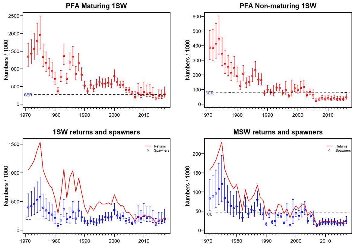
Figure 6 Top panels: Pre-Fisheries Abundance of Irish 1SW and MSW salmon stocks (red points with 95% confidence intervals) with respective Spawner Escapement Reserve indicated (dahed line). Bottom panels: Estimated return of 1SW and MSW salmon to Ireland prior to homewater fisheries (solid red line) and spawners (blue points with 95% confidence intervals) relative to respective national CL (dashed line). (source: ICES 2018).
