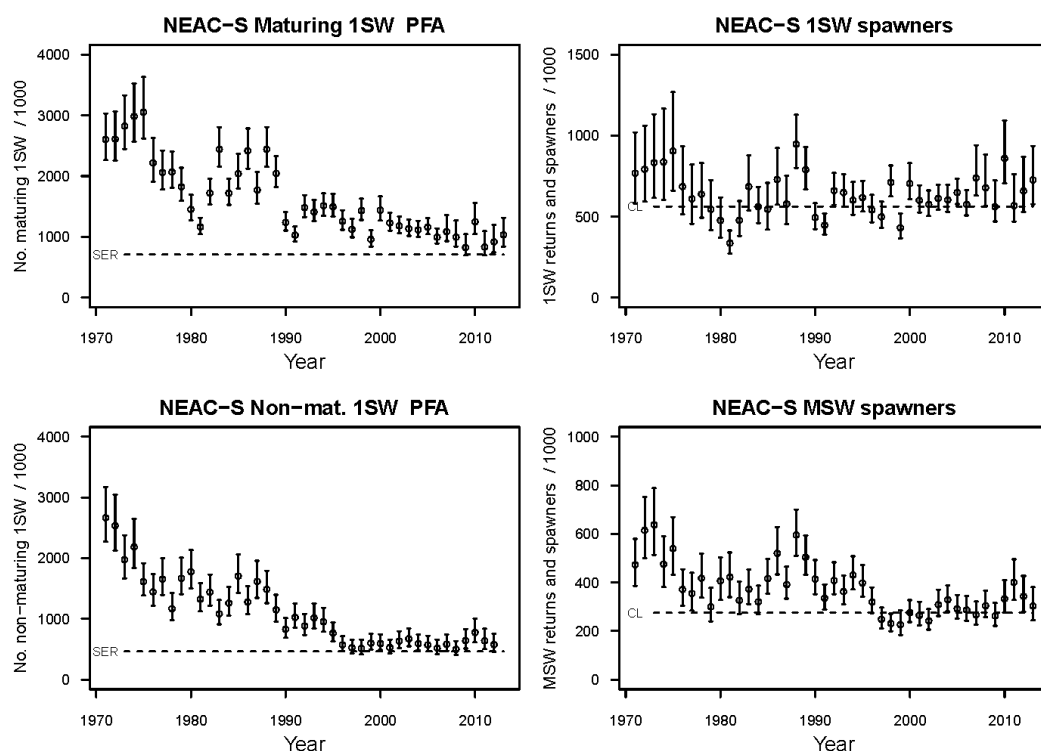
(Figure 2). Estimated PFA (left panels) and spawning escapement (right panels) with 90% confidence limits, for maturing 1SW (1SW spawners) and non-maturing 1SW (MSW spawners) salmon in southern NEAC (NEAC – S) stock complexes. (ICES CM 2014/ACOM:09)
