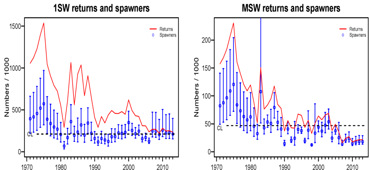
Figure 7. Estimated return of salmon to Ireland prior to homewater fisheries (solid line) and spawners (points including 95% confidence intervals) relative to National Conservation Limits (dashed line). Source ICES 2014.
