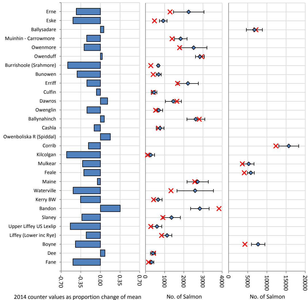
Figure 6. The proportional change in the salmon count in 2014 compared to previous multi-annual means (left panel), and mean salmon counts ( \pm 95% cls) with 2014 value indicated (red X) (middle and right panel – note the different axes scales).
