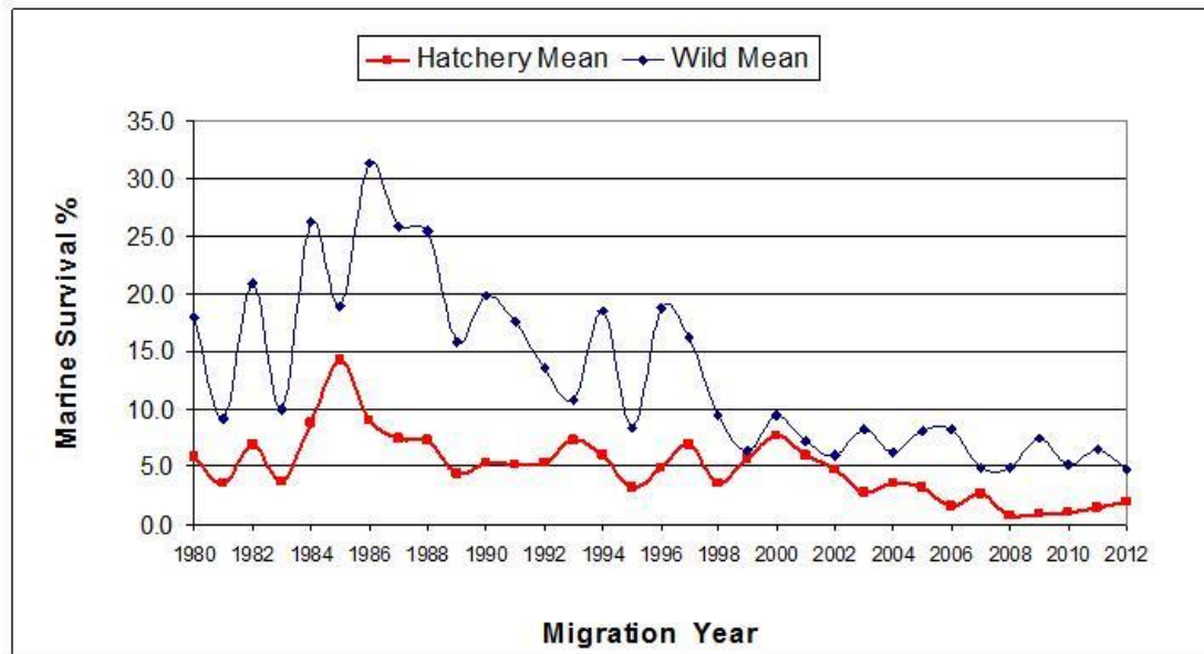
Figure 8. Marine survival (from smolt release to return to the coast) for wild and hatchery salmon.
