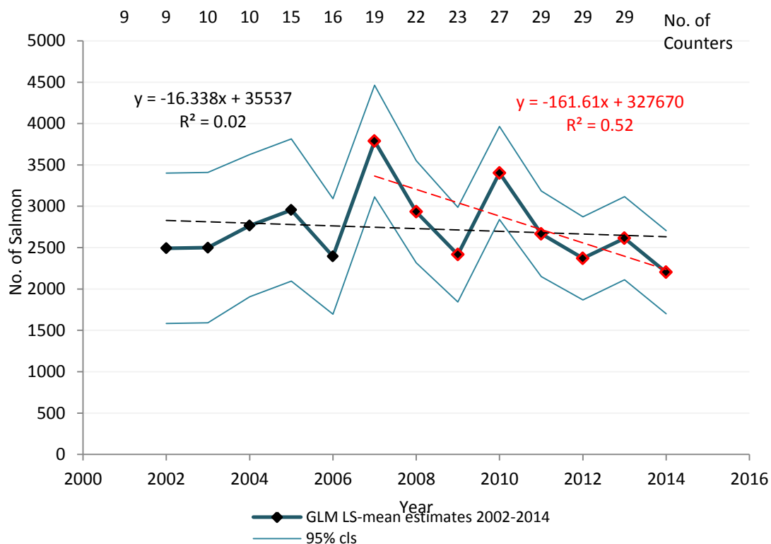
Figure 5. Marginal GLM LS-mean standardized number of salmon counted through counters operated between 2002 and 2014 ( \pm 95% cls - thin blue lines). The number of counters is shown at the top. The linear trend over the full time period (black dashed line), and between 2007 and the present (red dashed line) are also indicated. Note that the drift net fishery ceased at the end of the 2006 season.
