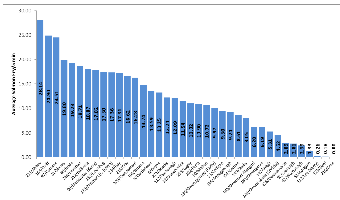
Figure VII -1. Results of catchment wide electro-fishing programme in 2014.
