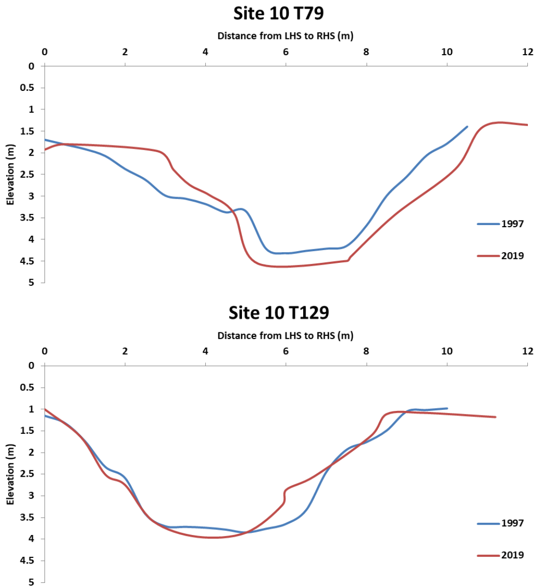
Figure 5.19 Cross-sectional form at two transects from Site 10 levelled in 1997 and 2019.
