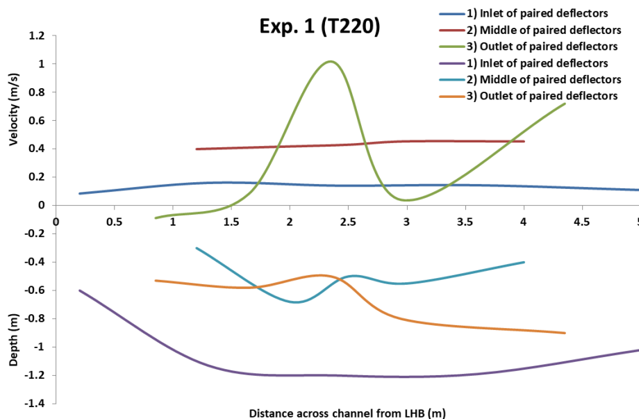
Figure 3.11 Depth velocity profile of paired deflectors located at T220 in Experimental site 1.
