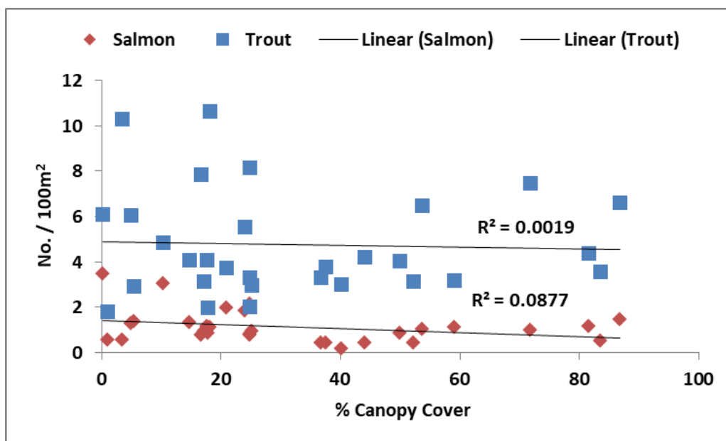
Figure 4.10 Percentage canopy cover vs fish density (numbers per 100m²) for brown trout and salmon.
