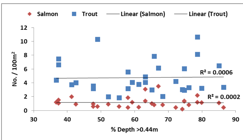
Figure 4.11 Depth >0.44m vs fish density (numbers per 100m²) for brown trout and salmon.
