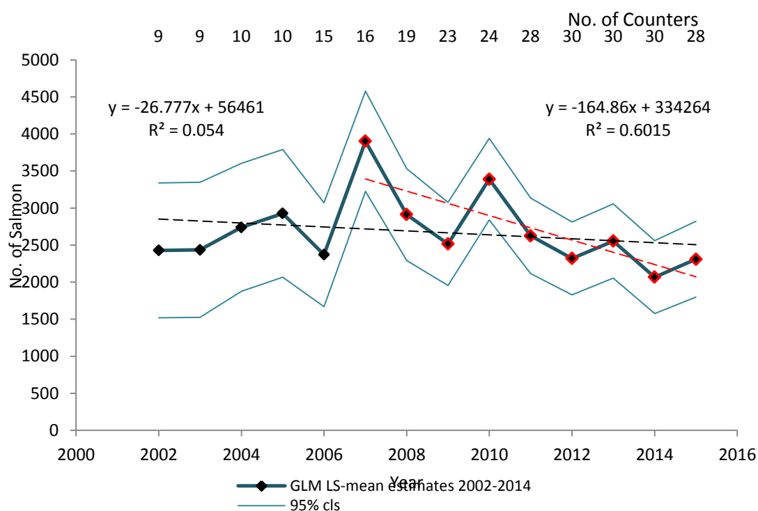
Figure 5. Marginal GLM LS-mean standardized number of salmon counted through counters operated between 2002 and 2015 ( \pm 95% cls - thin blue lines). The number of counters is shown at the top. The linear trend over the full time period (black dashed line), and between 2007 and the present (red dashed line) are also indicated. Note that the drift net fishery ceased at the end of the 2006 season.
