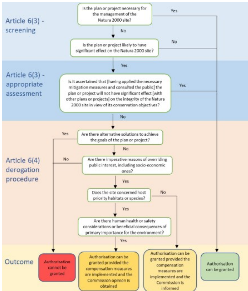
Figure 2: Appropriate Assessment stages
